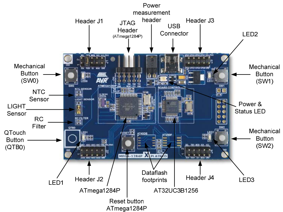
Figure 3-1. Overview of the MEGA-1284P Xplained kit.
