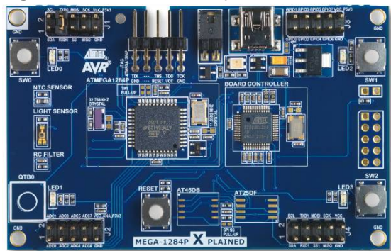
Figure 1-1. MEGA-1284P Xplained evaluation kit.
