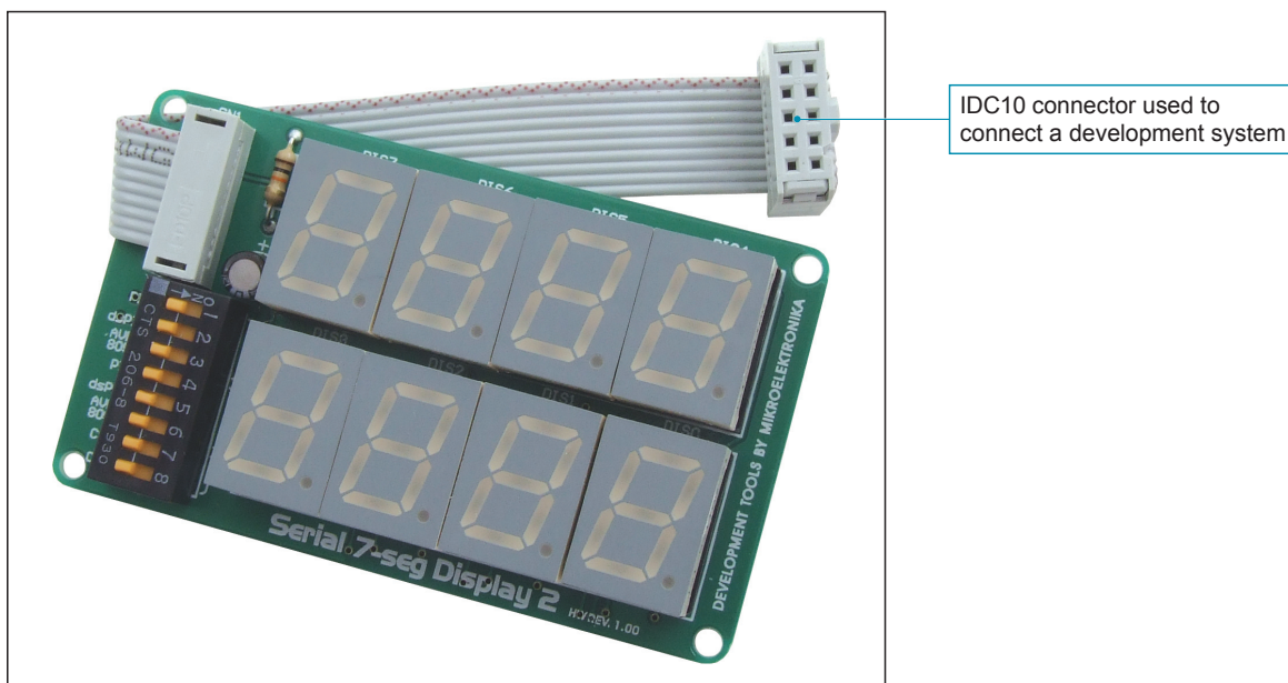
Figure 1: Serial 7-Seg Display 2 additional board
