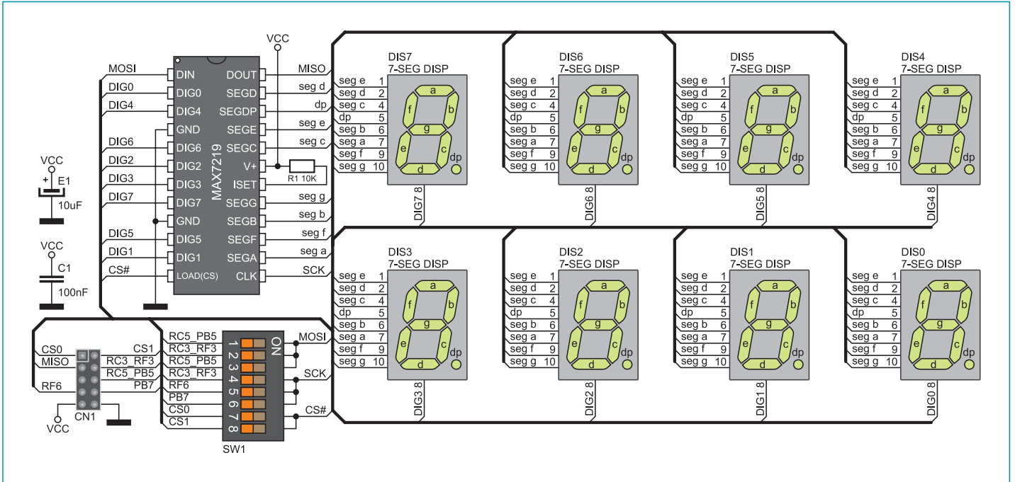
Figure 2: Serial 7-Seg Display 2 additional board connection schematic
