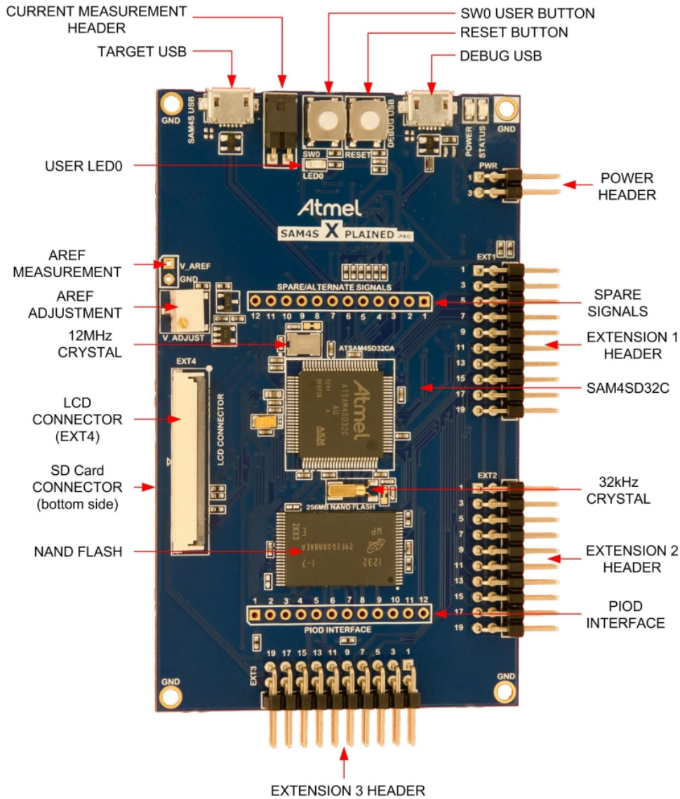
Figure 1.1. SAM4S Xplained Pro evaluation kit overview
