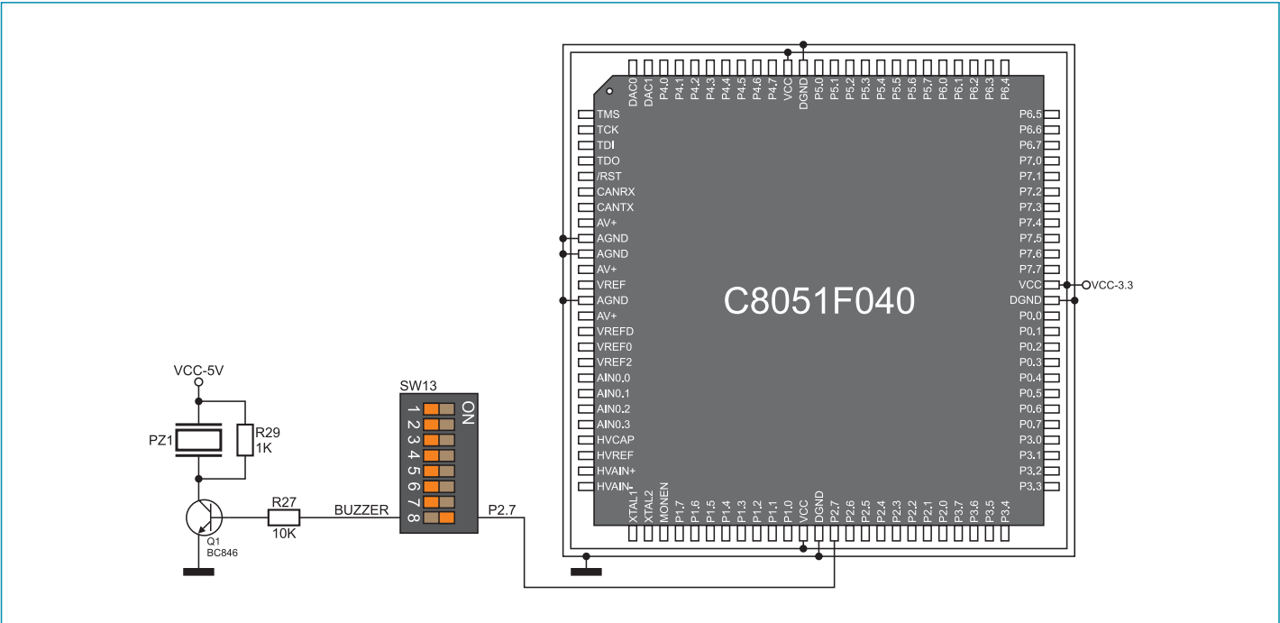
Figure 5-3: Piezo buzzer and microcontroller connection schematic
