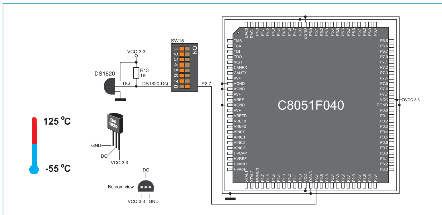
Figure 6-4: DS1820 and microcontroller connection schematic
