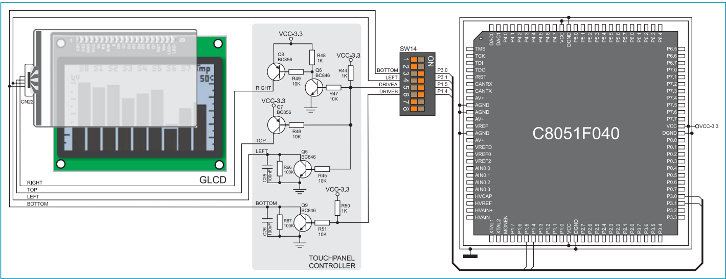
Figure 20-2: Touch panel connection schematic
