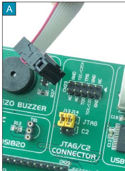
Figure 3-4: Connecting JTAG programmer with the development system
