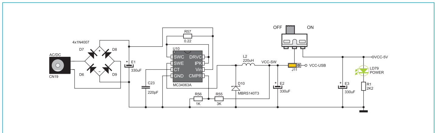
Figure 1-3: Power supply module connection schematic
