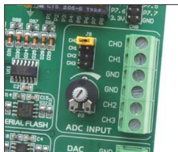
Figure 13-2: Jumper J9
