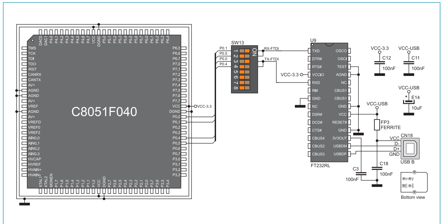
Figure 7-3: USB connector and microcontroller connection schematic
