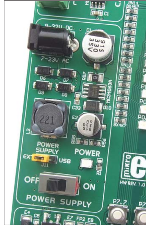
Figure 1-2: Power supply module
