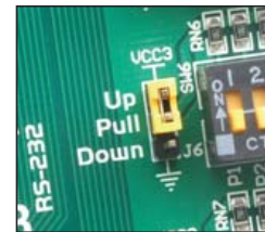
Figure 21-3: J9 in pull-up position
