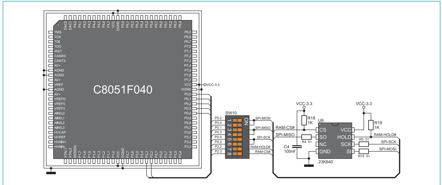
Figure 15-5: RAM module connection schematic
