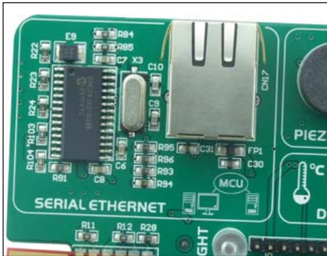
Figure 4-1: Ethernet module
