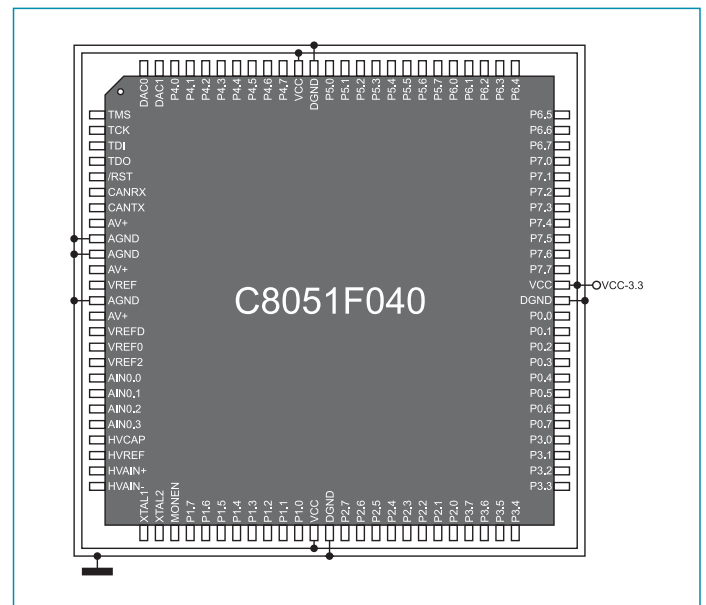
Figure 2-2: Microcontroller's pinout
