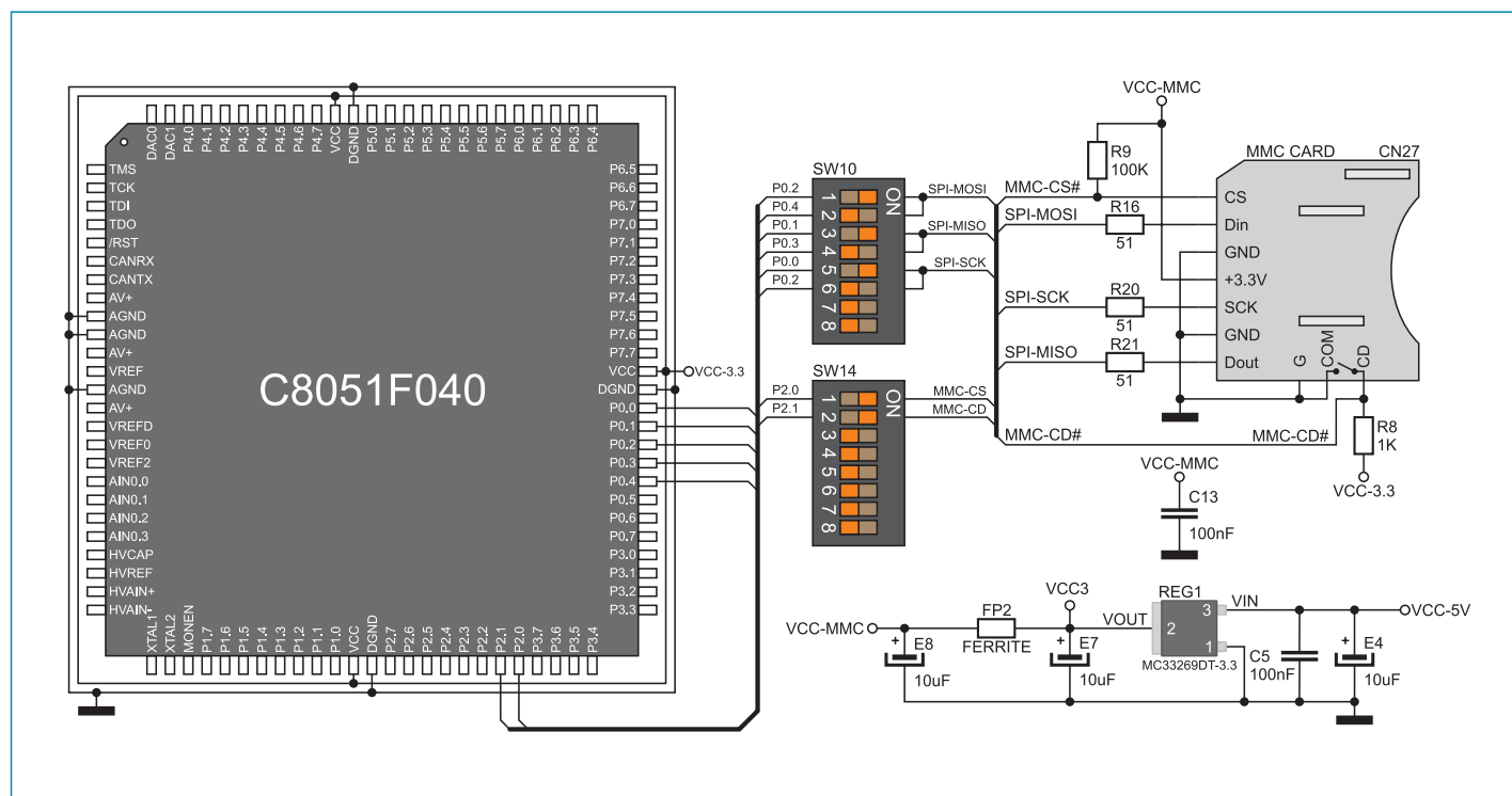
Figure 11-3: MMC/SD connector and microcontroller connection schematic
