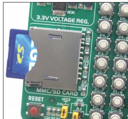
Figure 11-2: MMC/SD connector
