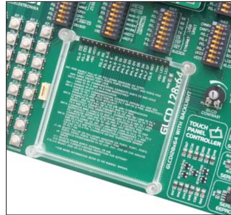
Figure 19-2: GLCD connector
