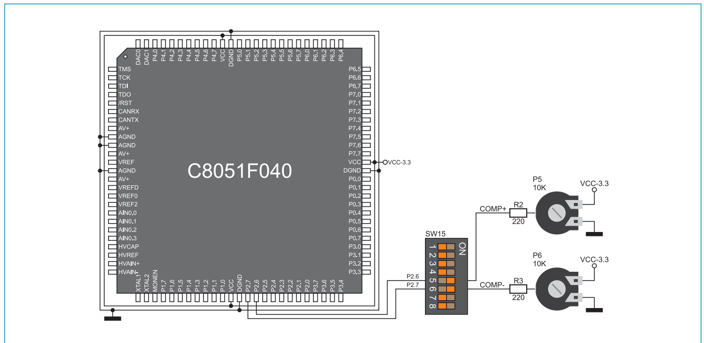
Figure 12-2: Comparator connection schematic
