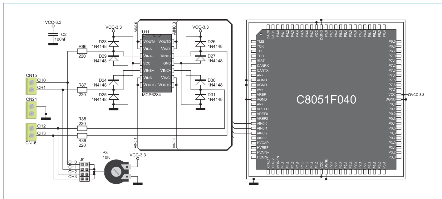
Figure 13-3: ADC module connection schematic
