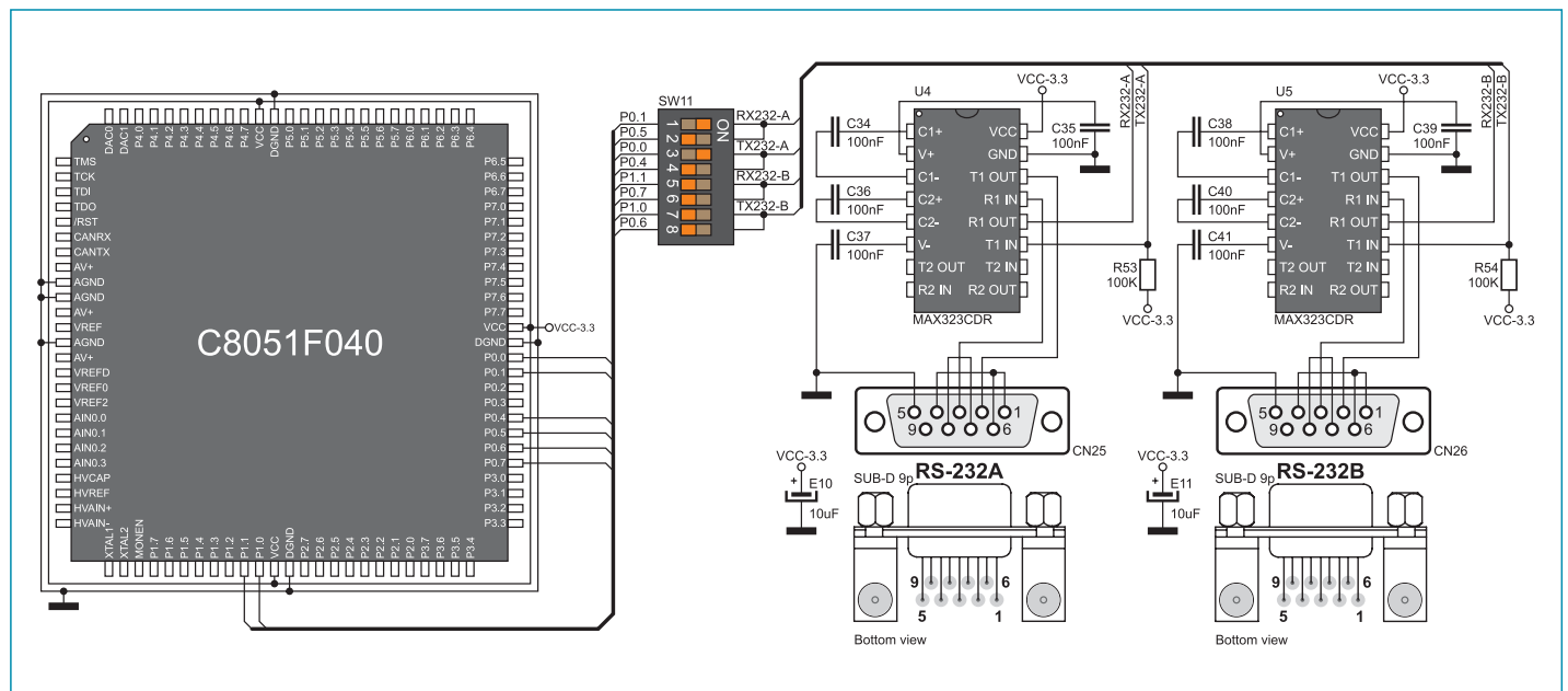
Figure 8-2: RS-232 module connection schematic
