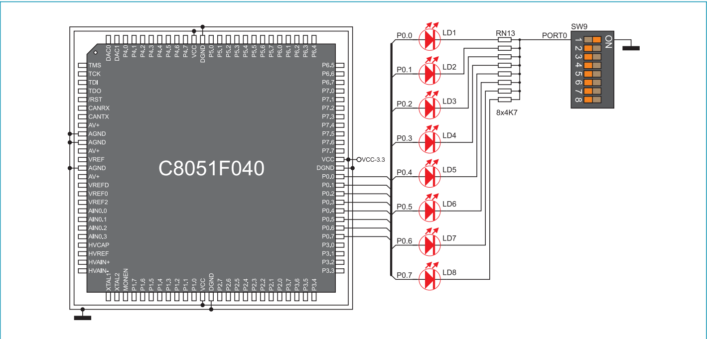
Figure 16-2: LED and port PORT0 connection schematic
