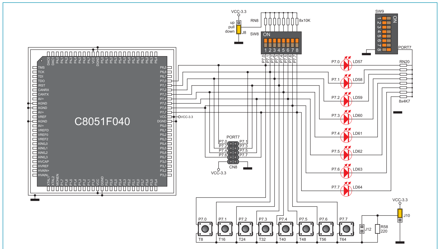
Figure 21-4: Port PORT7 connection schematic
