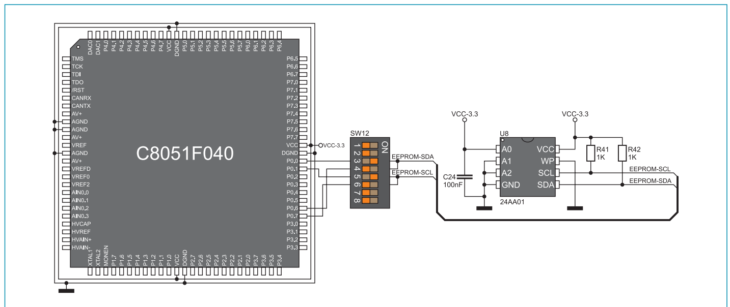
Figure 15-6: EEPROM module connection schematic
