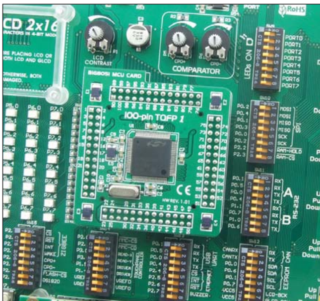
Figure 2-1: Microcontroller C8051F040
