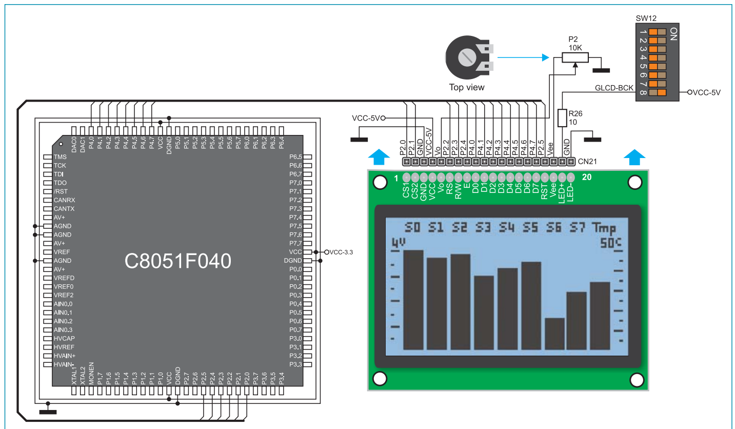
Figure 19-3: GLCD display connection schematic
