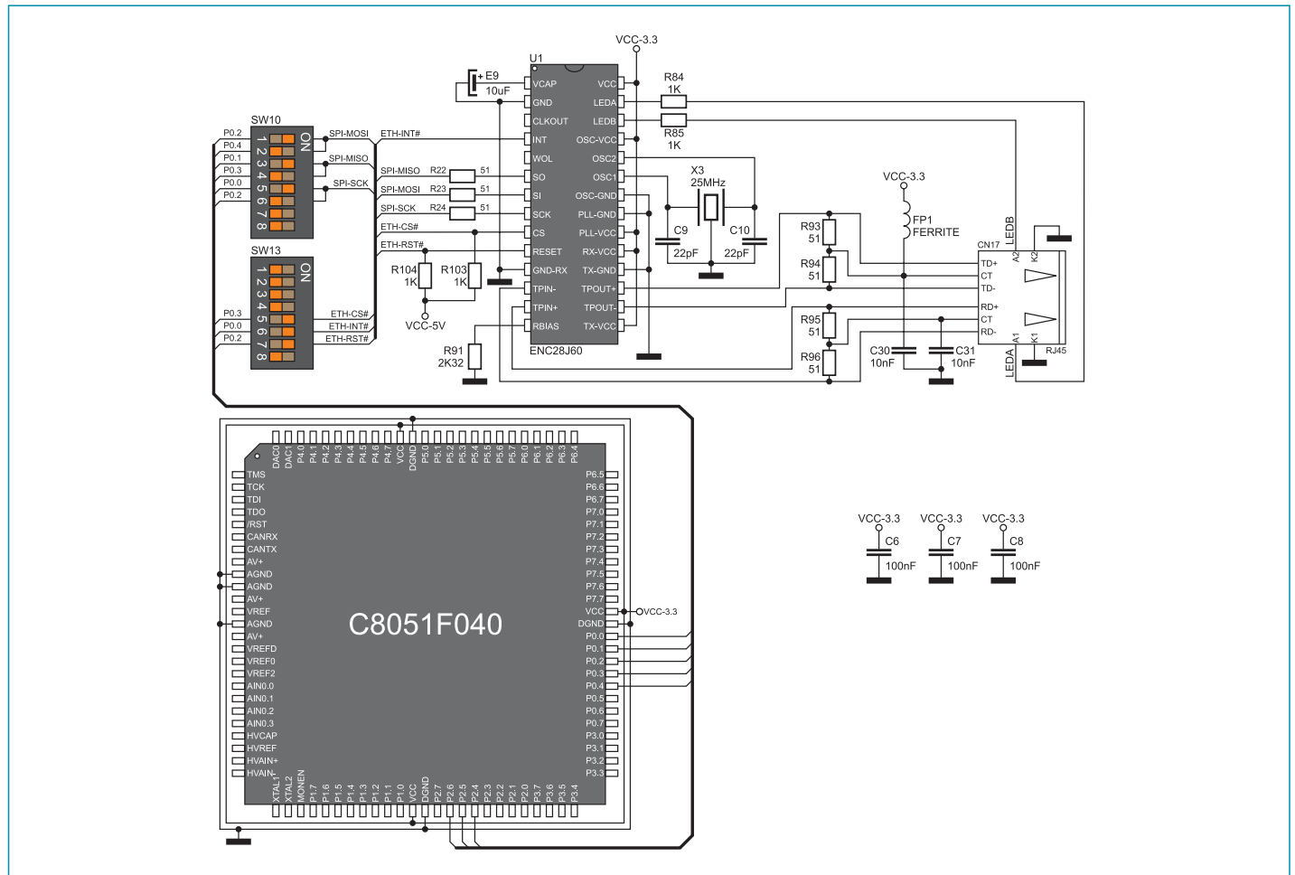
Figure 4-3: Ethernet module connection schematic
