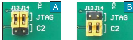
Figure 3-2: Position of jumpers 13 and 14
