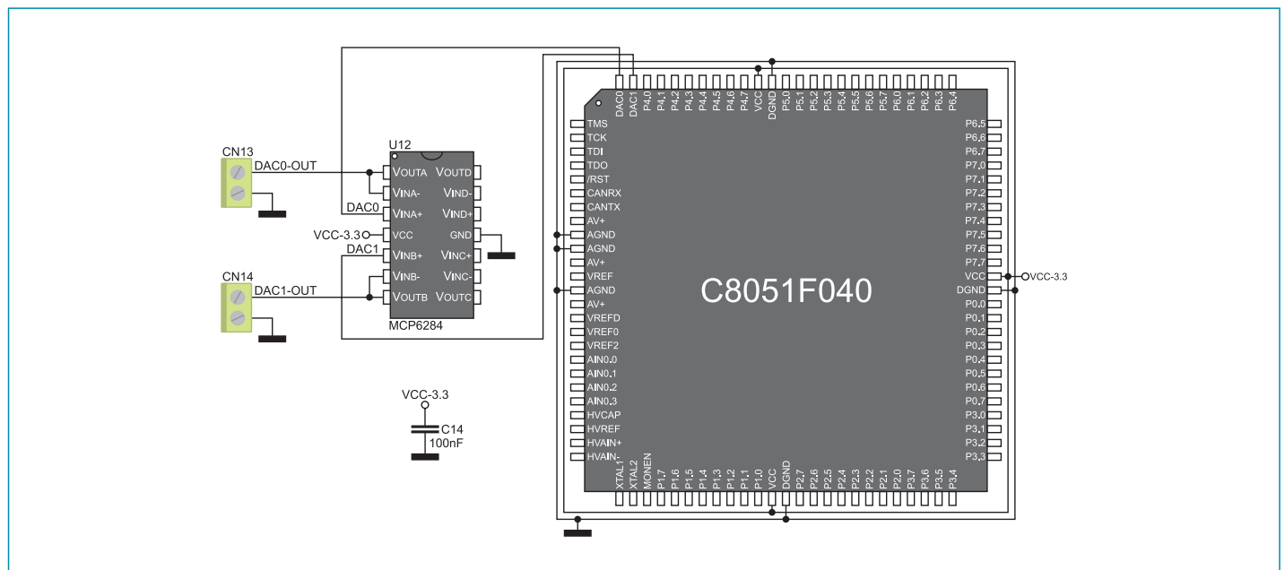
Figure 14-3: DAC module connection schematic
