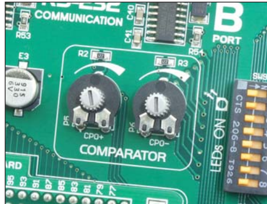
Figure 12-1: Comparator
