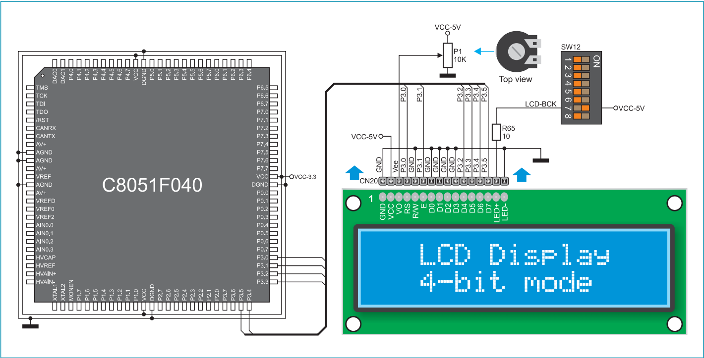
Figure 18-1: Connector for alphanumeric LCD display
