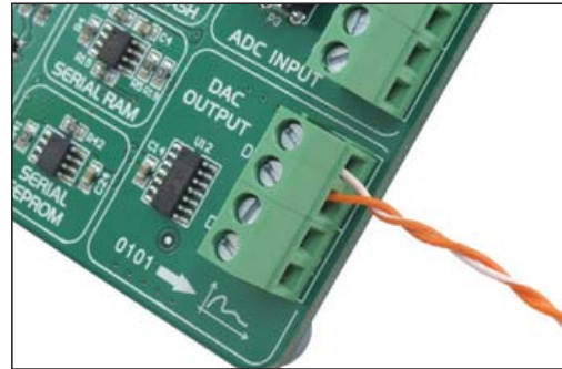
Figure 14-2: DAC module connector
