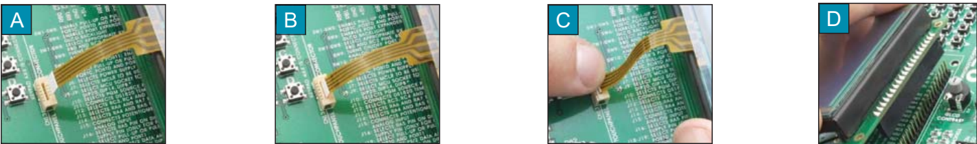
Figure 20-3: Connecting touch panel
