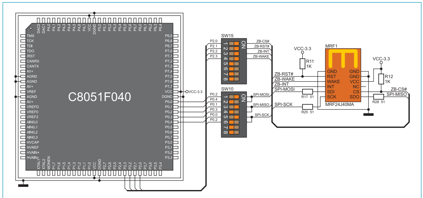
Figure 10-3: ZigBee module connection schematic
