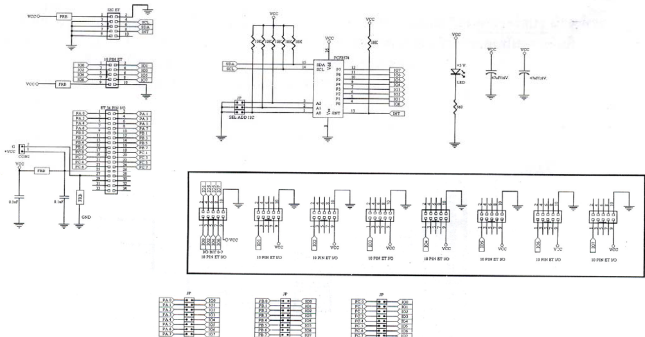
FIG 4: MR-BusIO-MAIN Schematic
