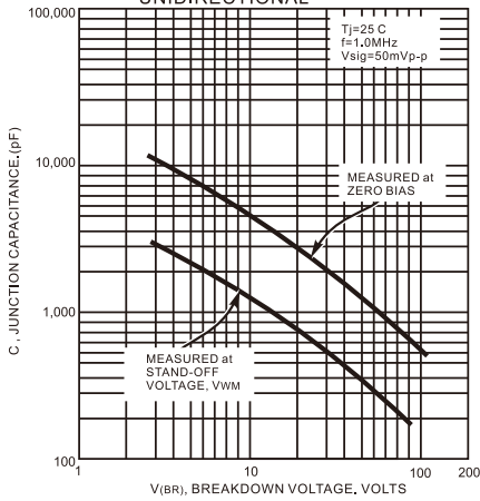
FIG.7- TYPICAL JUNCTION CAPACITANCE UNIDIRECTIONAL
