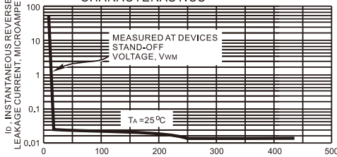
FIG.6- TYPICAL REVERSE LEAKAGE CHARACTERISTICS
