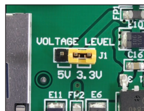
Figure 1-3: J1 in 3.3V position
