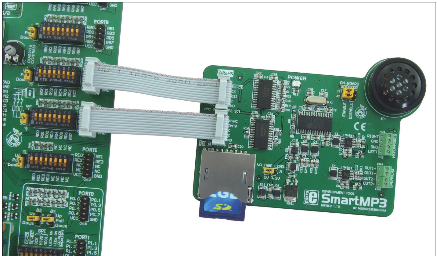
Figure 1-1: SmartMP3 connected to the development system
