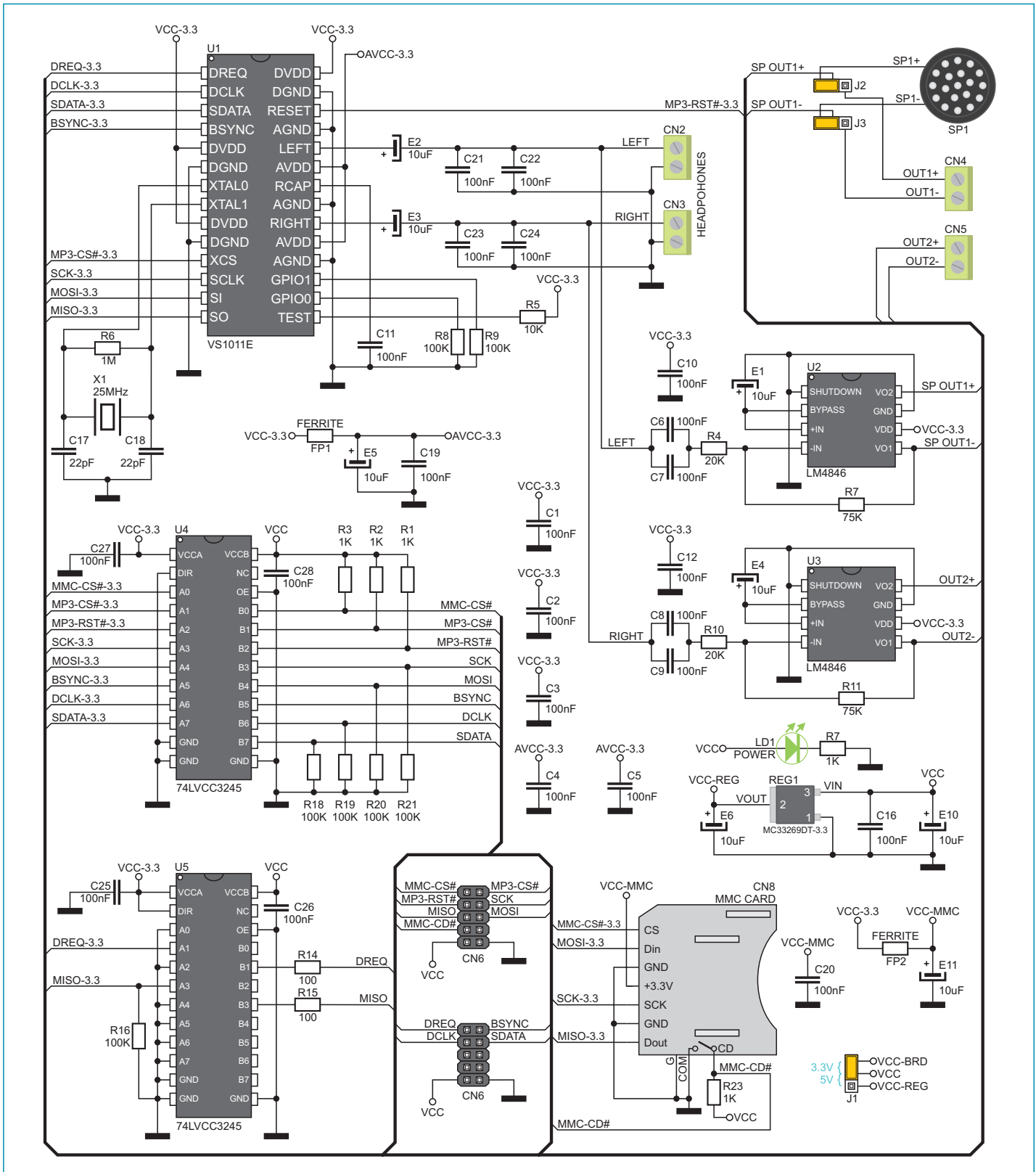
Figure 1-6: SmartMP3 additional board connection schematic
