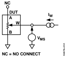
Figure 31. Resistor Integral Nonlinearity Error (Rheostat Operation; R-INL, R-DNL)
