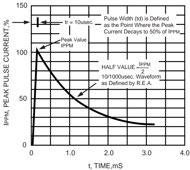
FIG. 3 - PULSE WAVEFORM
