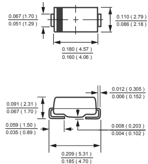
DO-214AC
