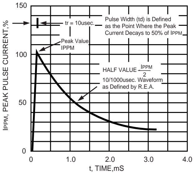
FIG. 3 - PULSE WAVEFORM
