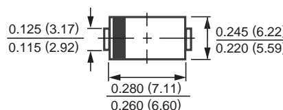
DO-214AB
