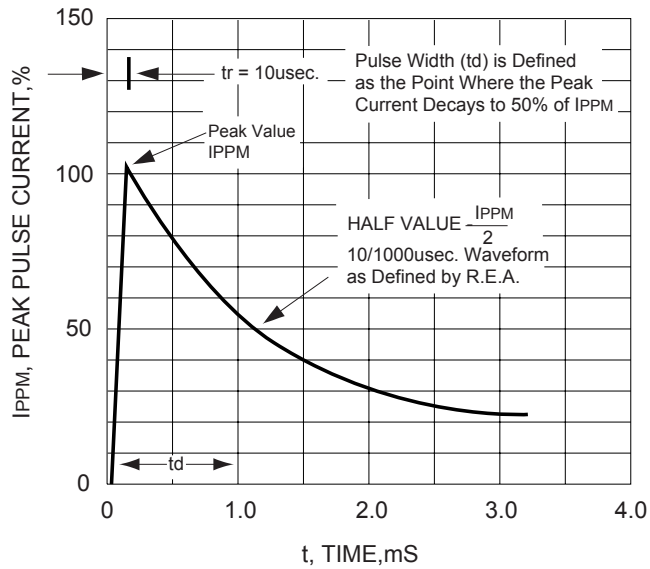
FIG. 3 - PULSE WAVEFORM
