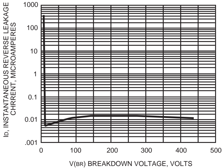
FIG. 7 - TYPICAL REVERSE LEAKAGE CHARACTERISTICS
