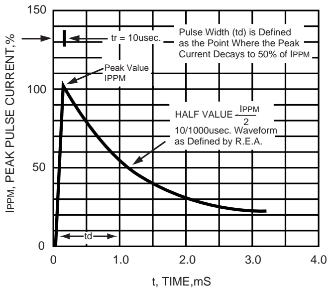
FIG. 3 - PULSE WAVEFORM
