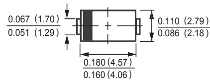
DO-214AC
