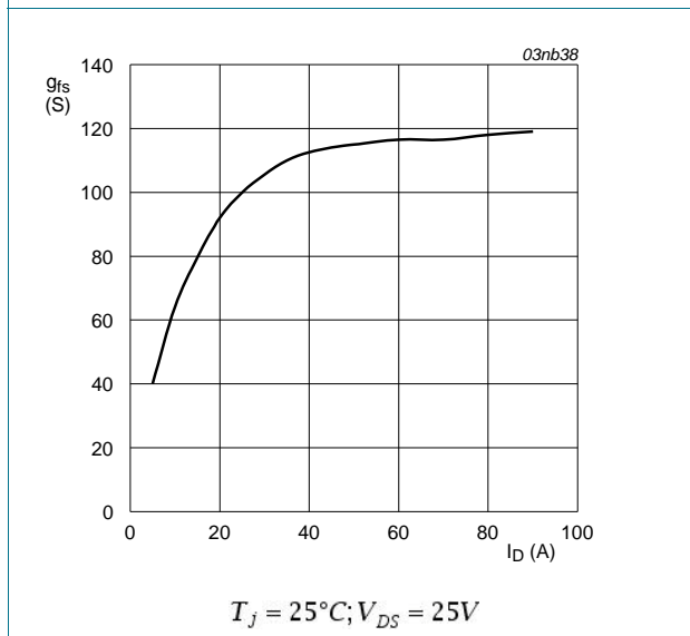
Fig 11. Forward transconductance as a function of drain current; typical values
