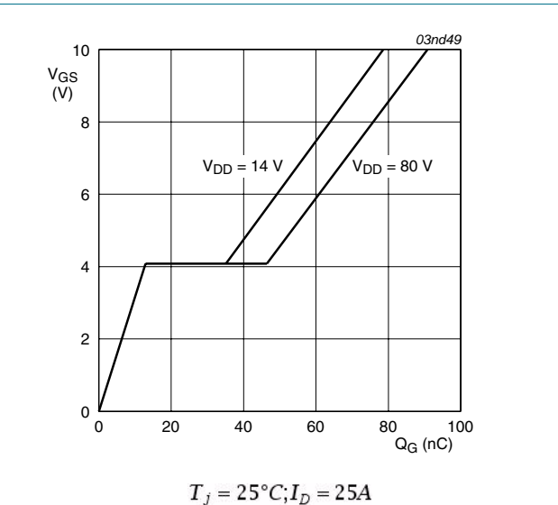
Fig 10. Gate-source voltage as a function of turn-on gate charge; typical values
