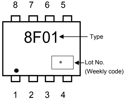
Figure 2 Marking (Note 3)
