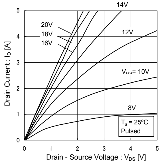
Fig.5 Typical Output Characteristics(II)
