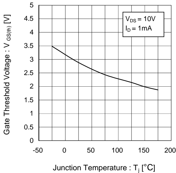
Fig.10 Gate Threshold Voltage vs. Junction Temperature
