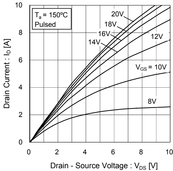
Fig.6 T_j = 150^\circ\text{C} Typical Output Characteristics(I)
