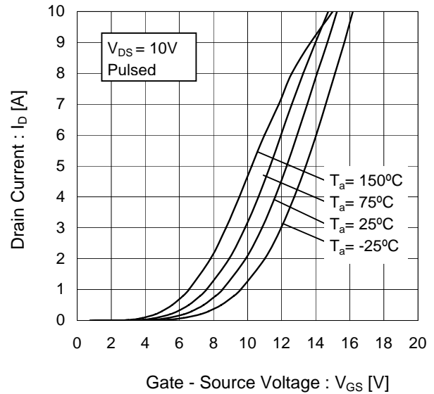
Fig.9 Typical Transfer Characteristics (II)
