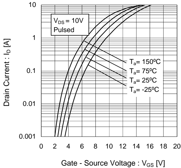
Fig.8 Typical Transfer Characteristics (I)
