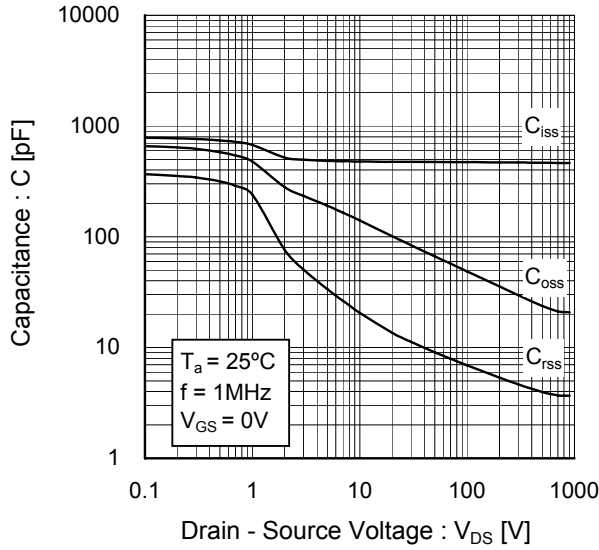
Fig.15 Typical Capacitance vs. Drain - Source Voltage
