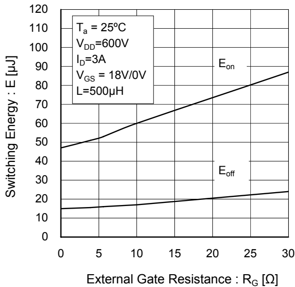
Fig.21 Typical Switching Loss vs. External Gate Resistance
