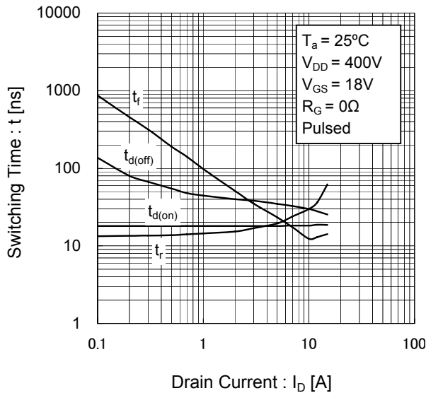
Fig.17 Switching Characteristics
