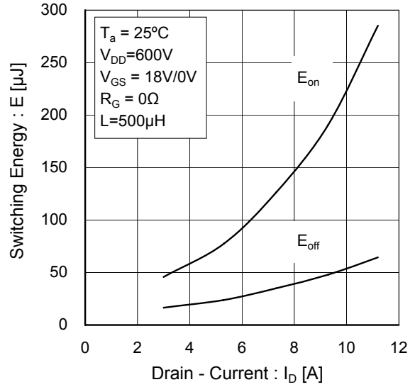
Fig.20 Typical Switching Loss vs. Drain Current
