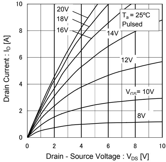
Fig.4 Typical Output Characteristics(I)
