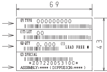
Reel label, Inner box label (unit:mm)
