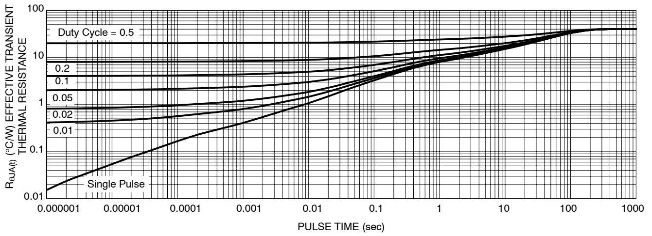
Figure 12. Thermal Response
