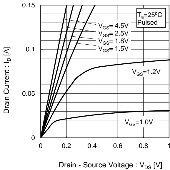
Fig.3 Typical Output Characteristics(I)
