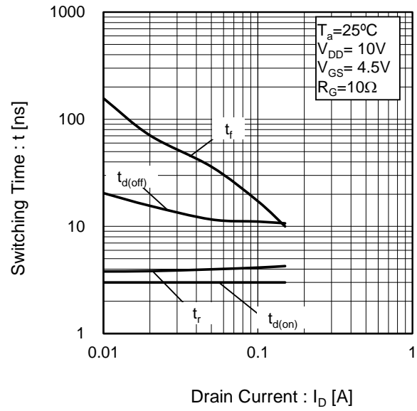
Fig.18 Switching Characteristics
