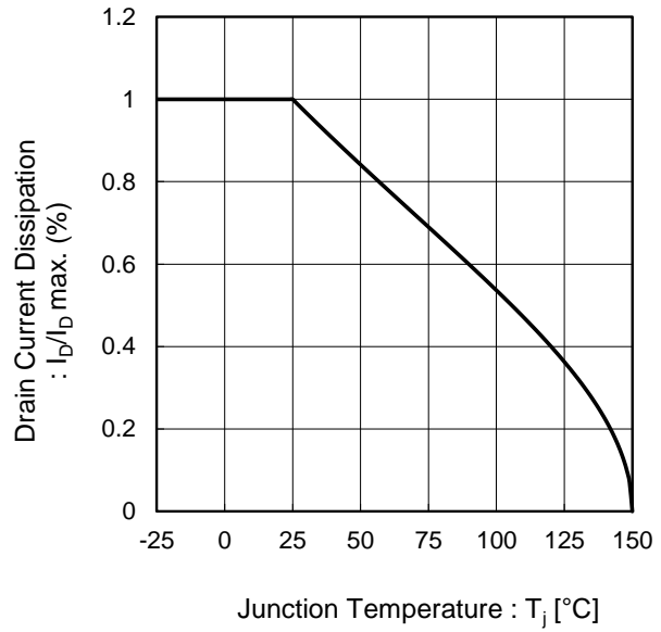
Fig.2 Drain Current Derating Curve
