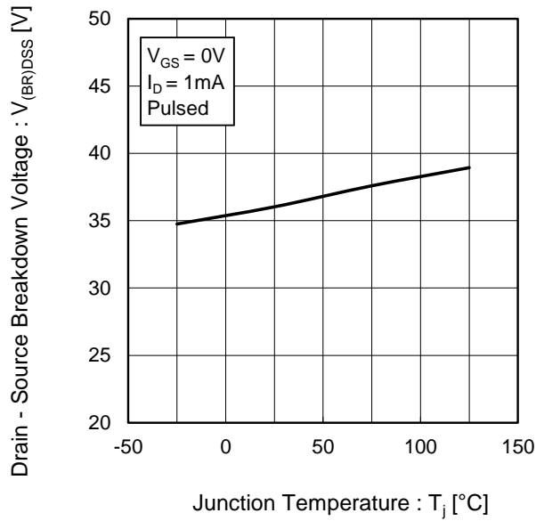
Fig.5 Breakdown Voltage vs. Junction Temperature
