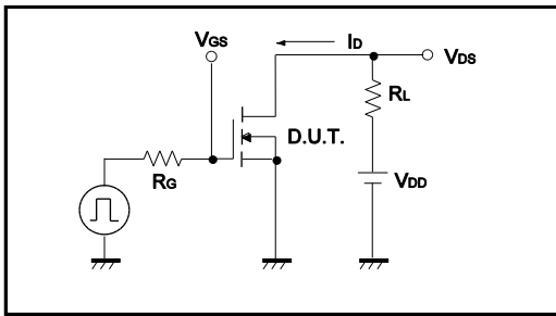
Fig.1-1 Switching Time Measurement Circuit
