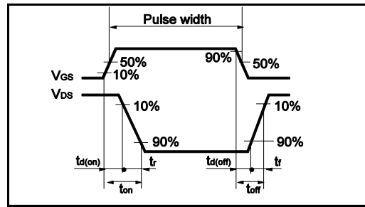
Fig.1-2 Switching Waveforms
