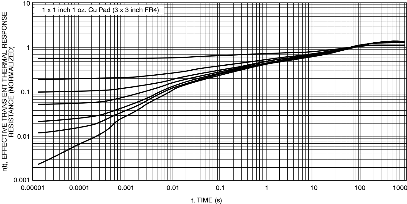
Figure 13. Thermal Response
