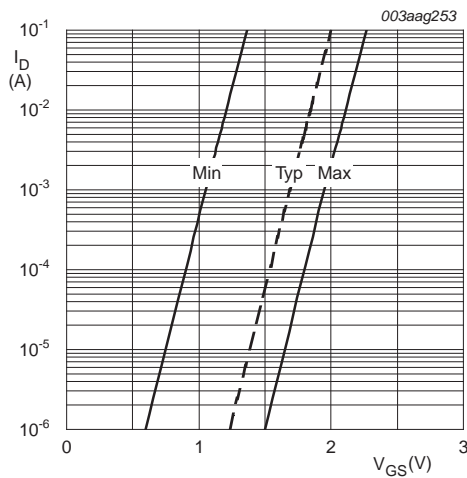
T_j = 25^\circ C; V_{DS} = 5V
