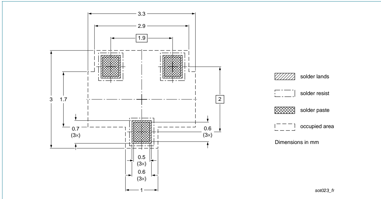
Fig 19. Reflow soldering footprint for SOT23 (TO-236AB)
