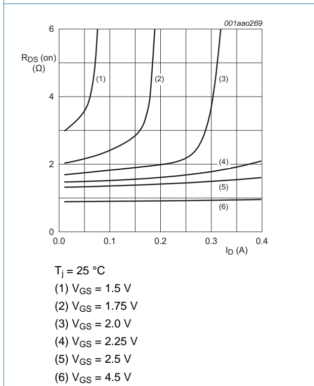
Fig 11. TR1: Drain-source on-state resistance as a function of drain current; typical values
