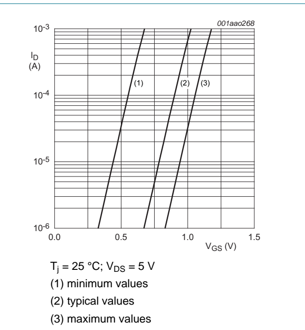
Fig 10. TR1: Sub-threshold drain current as a function of gate-source voltage
