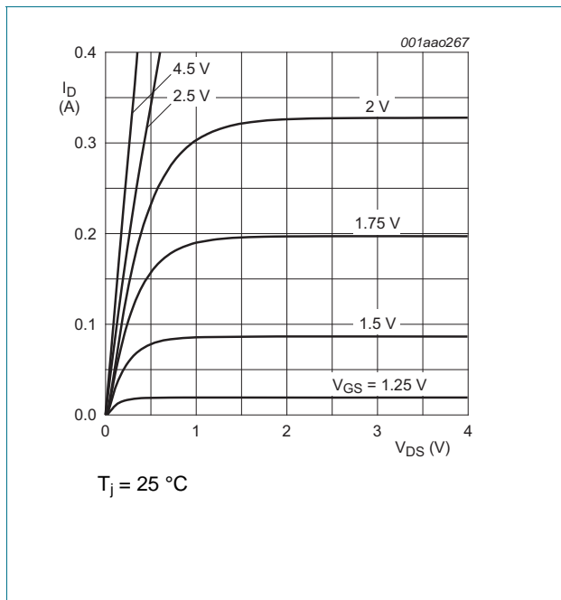
Fig 9. TR1: Output characteristics: drain current as a function of drain-source voltage; typical values
