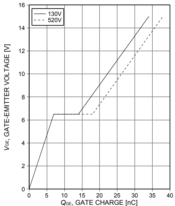
Figure 16. Typical gate charge ( I_C=15\text{A} )
