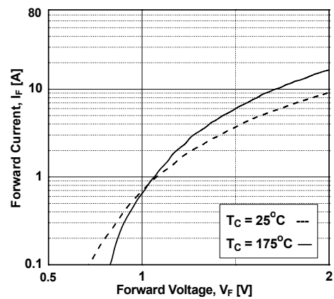
Figure 18. Forward Characteristics
