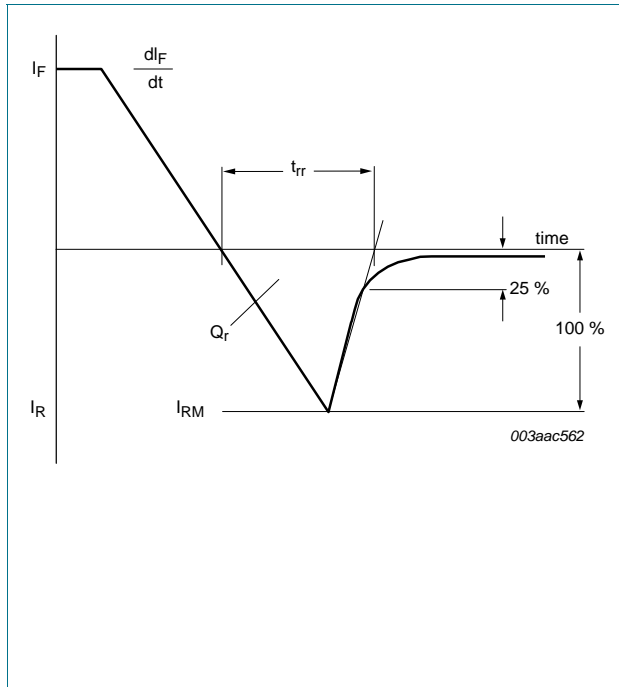
Fig 6. Reverse recovery definitions; ramp recovery
