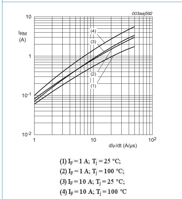
Fig 8. Peak reverse recovery current as a function of rate of change of forward current; maximum values
