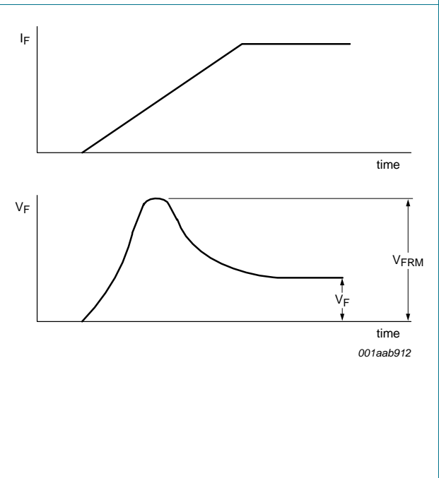
Fig 9. Forward recovery definitions
