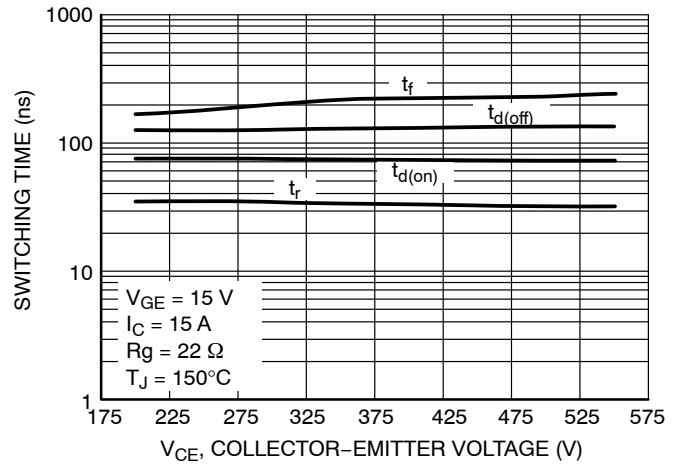
Figure 16. Switching Time vs. Collector-Emitter Voltage
