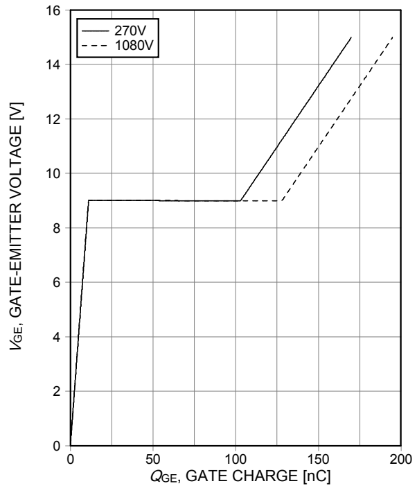
Figure 18. Typical gate charge ( I_C=20\text{A} )
