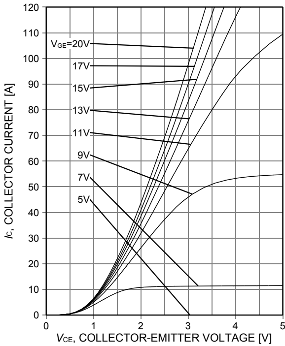
Figure 5. Typical output characteristic ( T_j=175^\circ\text{C} )
