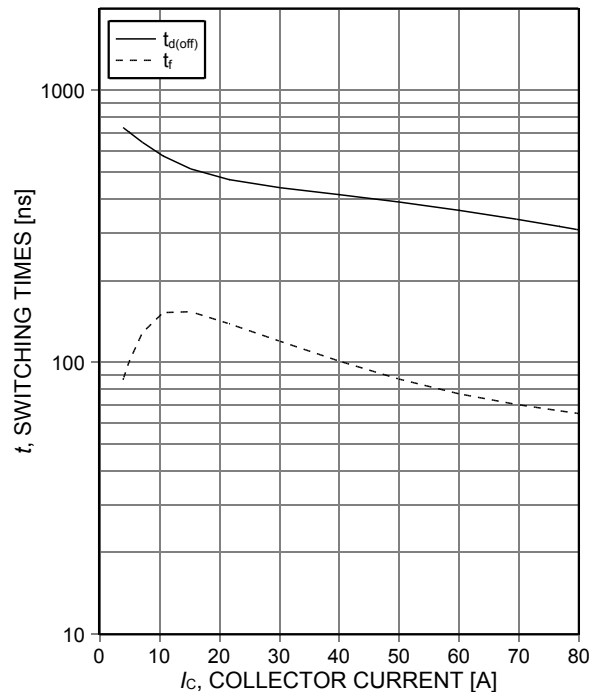
Figure 8. Typical switching times as a function of collector current (inductive load, T_j=175^\circ\text{C} , V_{CE}=600\text{V} , V_{GE}=15/0\text{V} , r_G=7,5\Omega , Dynamic test circuit in Figure E)
