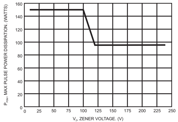
FIG.4- MAXIMUM PULSE POWER DISSIPATION vs ZENER VOLTAGE
