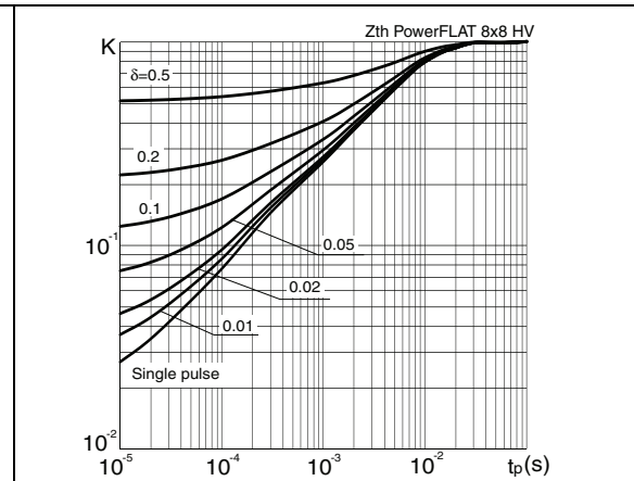
Figure 3. Thermal impedance
