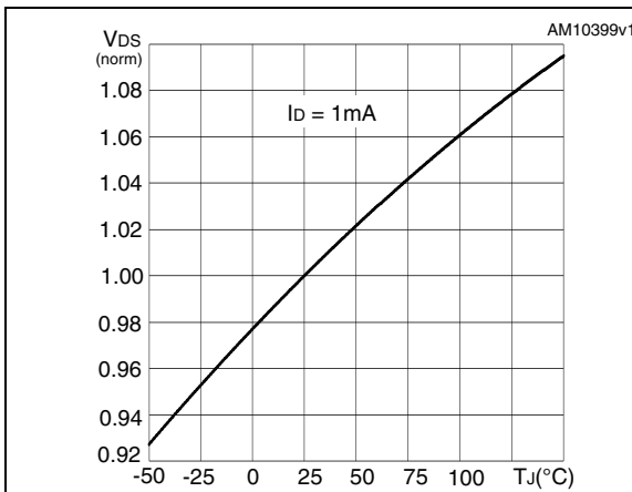
Figure 12. Normalized BVDS vs temperature
