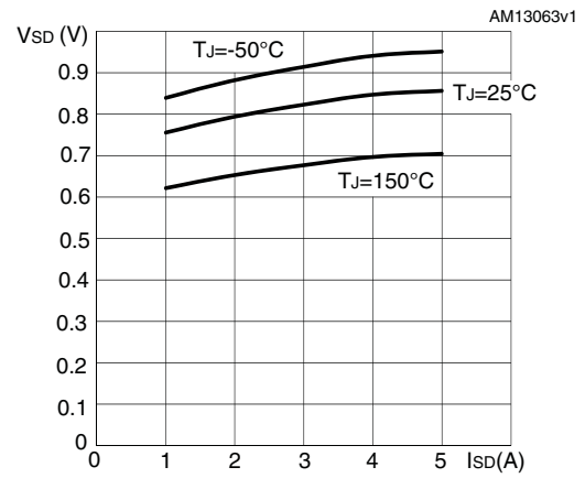
Figure 15. Source-drain diode forward characteristics
