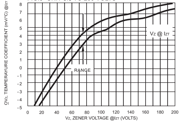
FIG.5- UNIT 6.8 TO 200 VOLTS
