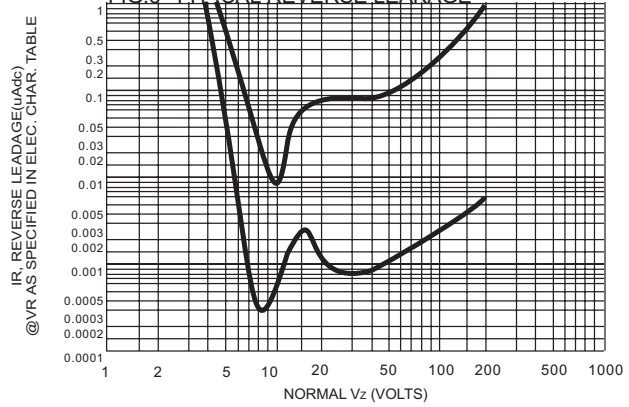
FIG.5- UNIT 6.8 TO 200 VOLTS
