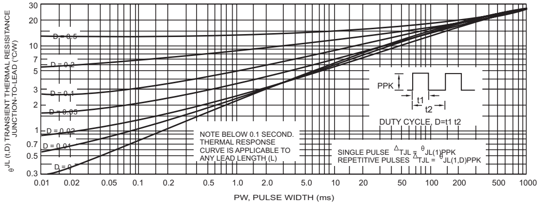
FIG.2- MAXIMUM SURGE POWER
