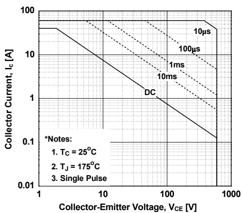
Figure 11. SOA Characteristics
