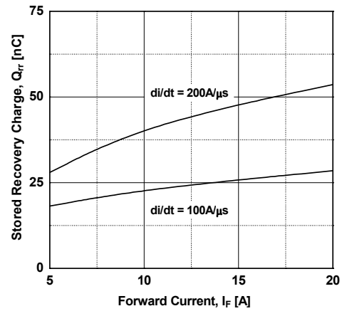
Figure 24. Stored Charge
