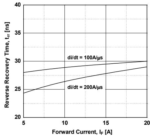
Figure 25. Reverse Recovery Time
