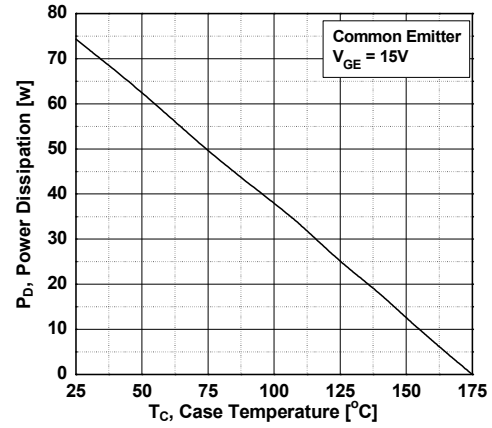
Figure 20. Power Dissipation
