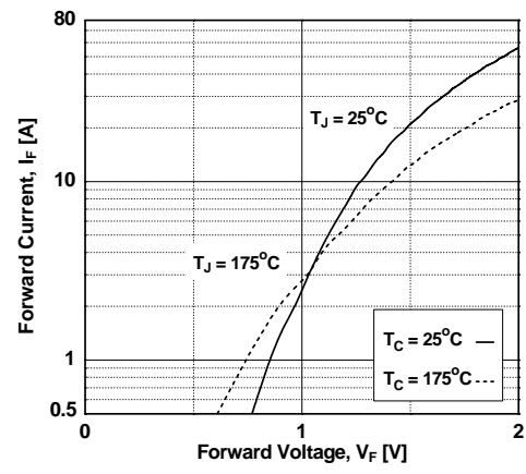
Figure 18. Forward Characteristics
