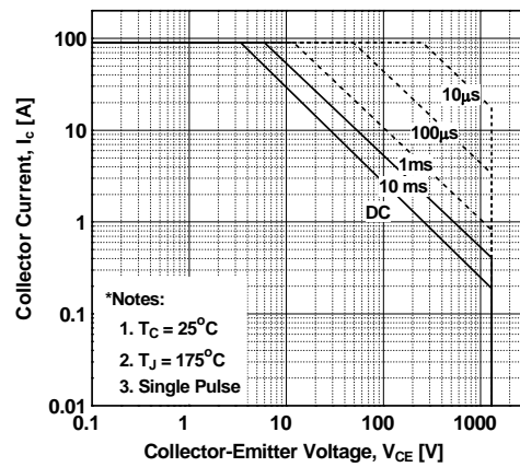
Figure 10. SOA Characteristics
