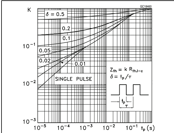
Figure 14. Thermal impedance
