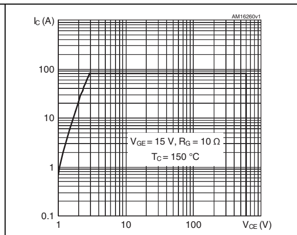
Figure 13. Turn-off SOA
