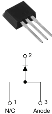
TO-262
