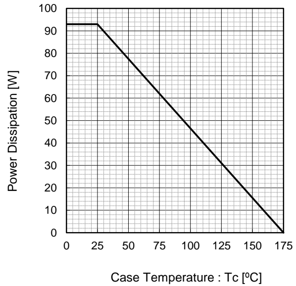
Fig.6 Power Dissipation
