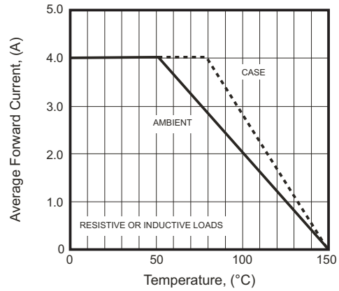
Fig.2 - Forward Derating Current
