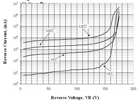
Fig. 4 Reverse Current vs Reverse
