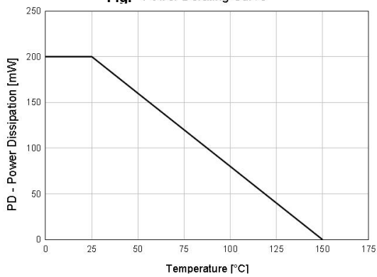
Fig. Power Derating Curve
