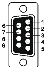
Figure 1: Pin locations for Serial Port Connector (Port 1)
