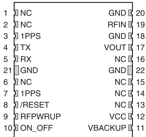
Figure 5: R4 Series GPS Receiver Pinout (Top View)
