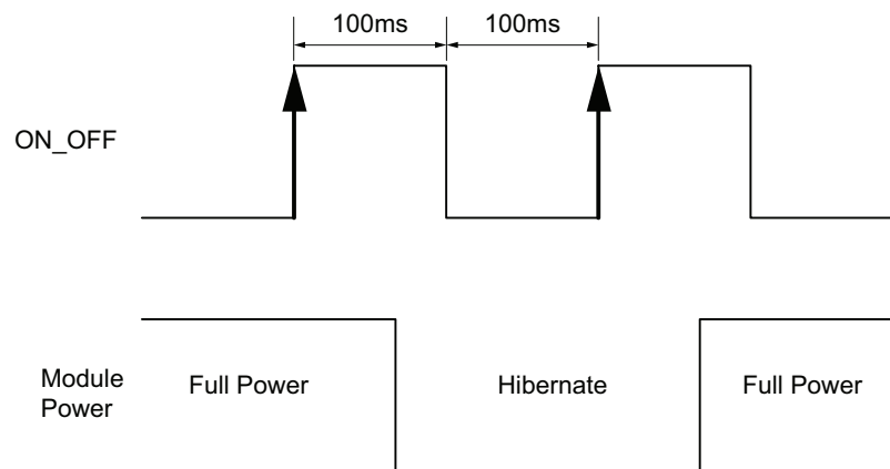
Figure 7: R4 Series GPS Receiver Power Control
