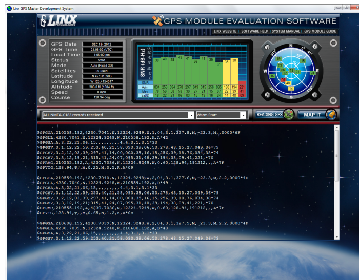
Figure 30: The R4 Series Master Development System Software
