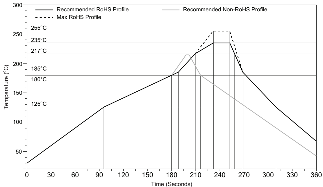
Figure 36: Maximum Reflow Profile
