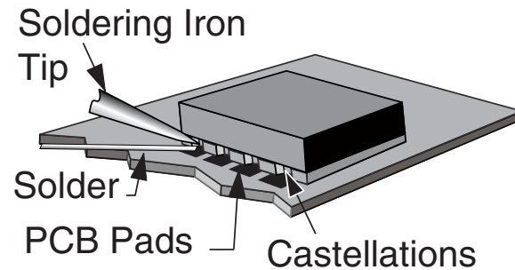
Figure 34: Soldering Technique
