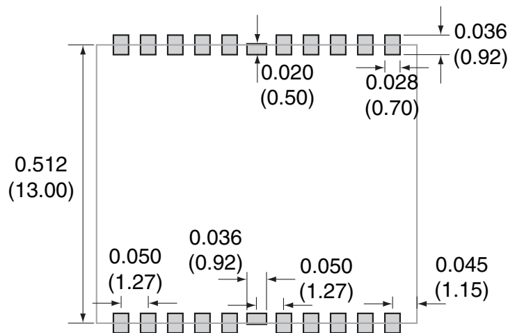
Figure 31: Recommended PCB Layout
