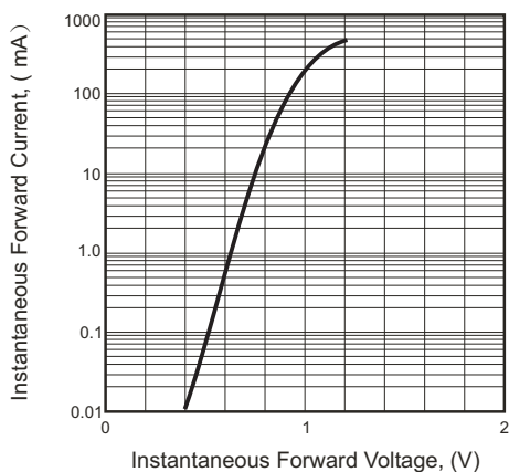
Fig.5 - Forward Characteristics
