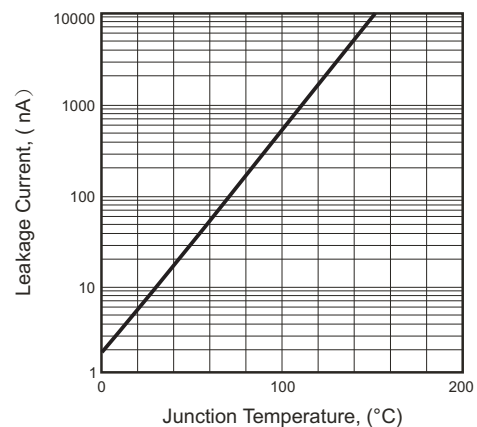
Fig.6 - Leakage Current vs Junction Temperature
