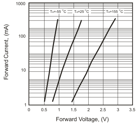
Fig.1 - Forward Characteristics
