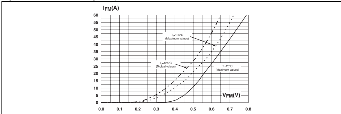
Figure 9. Forward voltage drop versus forward current
