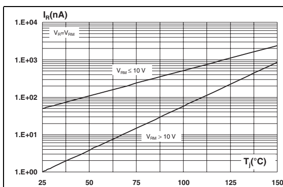
Figure 14. Leakage current versus junction temperature (typical values)
