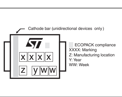
Figure 18. Marking layout (1)
