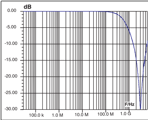
Figure 11. S21 attenuation measurement
