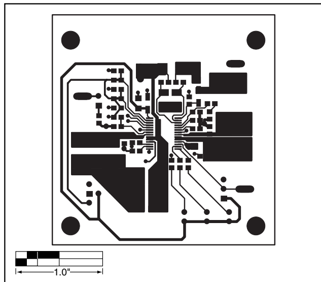
Figure 3. MAX1757/MAX1758 EV Kit PC Board Layout—Component Side
